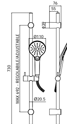
ZSAL 210CR SOFIA Saliscendi Sofia con doccia (2 getti) in ABS Sofia sliding rails with (2-spray functions) ABS hand-shower
