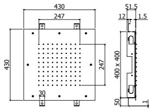
ZSOF 300CR NEW YORK Soffione ad incasso "Quadro" in metallo, anticalcare - 430x430 mm "Square" concealed ceiling metal shower head, antiscalc system - 430x430 mm
