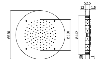
ZSOF 304CR LAS VEGAS Soffione ad incasso "Tondo" in metallo, anticalcare - Ø 550 mm "Round" concealed ceiling metal shower head, antiscalc system - Ø 550 mm
