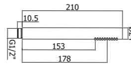
ZDOC 067CR MASTER Doccia Master (monogetto) in metallo Master (single-spray) metal hand-shower
