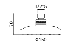
ZSOF 029CR ARIZONA Soffione "Arizona" in ABS, anticalcare Ø 150 mm "Arizona" ABS shower head, antiscala system - Ø150 mm
