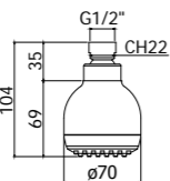
ZSOF 031CR ALABAMA Soffione "Alabama" in ABS, anticalcare Ø 70 mm "Alabama" ABS shower head, antiscald system - Ø 70 mm
