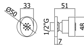
ZSOF 073CR Soffione ellittico in metallo, anticalcare - 48x33 mm Oval metal body jet, antiscaling system - 48x33 mm
