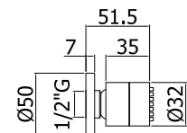
ZSOF 061CR Soffione tondo in metallo, anticalcare - Ø32 mm Round metal body jet, antiscaling system - Ø32 mm
