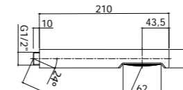
ZDOC 032CR BIRILLO Doccia Birillo (monogetto) in ABS Birillo (single-spray) ABS hand-shower
