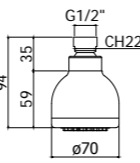
ZSOF 032CR OREGON Soffione "Oregon" in ABS, anticalcare Ø 70 mm "Oregon" ABS shower head, antiscald system - Ø 70 mm
