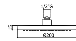
ZSOF 115CR PANDA Soffione "Panda" in ABS, anticalcare Ø 200 mm "Panda" ABS shower head, antiscala system Ø 200 mm
