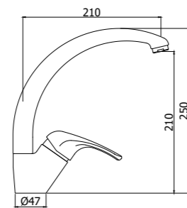
ND 181CR Miscelatore lavello monoforo con canna tubo orientabile One-hole sink mixer with tube swivelling spout
