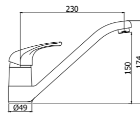
ND 182CR Miscelatore lavello monoforo canna fusa orientabile One-hole sink mixer with swivelling cast spout
