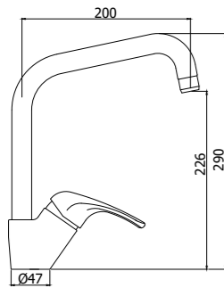
ND 180CR Miscelatore lavello monoforo con canna tubo orientabile One-hole sink mixer with tube swivelling spout
