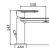
CA 071-075CR Miscelatore lavabo con/senza scarico Wash basin mixer with/without pop up waste
