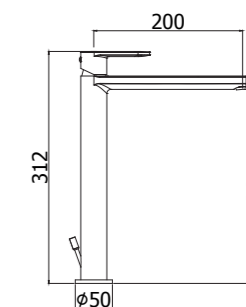
CA 081-085CR Miscelatore lavabo prolungato con/senza scarico Tall wash basin mixer with/without pop up waste
