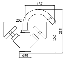
QTV 138-137CR Monoforo bidet con/senza scarico One-hole bidet mixer with/without pop up waste
