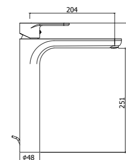
GR 081-085CR Miscelatore lavabo prolungato con/senza scarico Tall wash basin mixer with/without pop up waste
