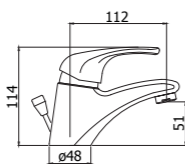
ND 071-075CR Miscelatore lavabo con/senza scarico Wash basin mixer with/without pop up waste
