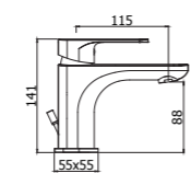
SY 071-075CR-ES Con cartuccia ENERGY SAVING With ENERGY SAVING cartridge
