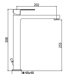
EL 081-085CR Miscelatore lavabo prolungato con/senza scarico Tall wash basin mixer with/without pop up waste
